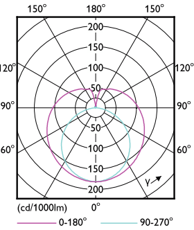
Light Distribution Diagram - 9.5T8/MAS/48-850/MF18/G/DIM UE 25/1
