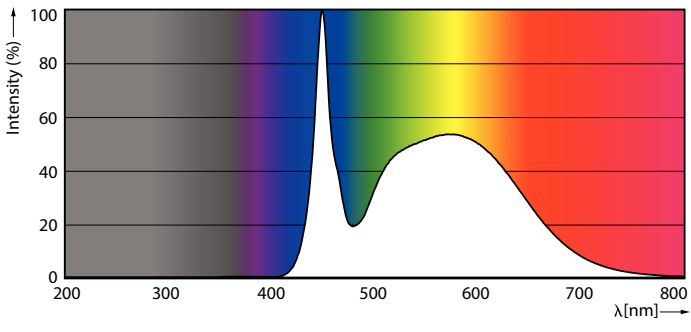
Spectral Power Distribution Colour - 9.5T8/MAS/48-850/MF18/G/DIM UE 25/1
