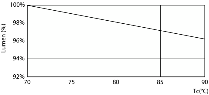
Lumen Maintenance Diagram - 9.5T8/MAS/48-840/MF18/G/DIM UE 25/1
