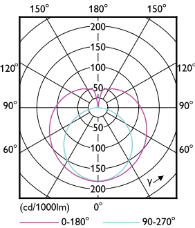
Light Distribution Diagram - 9.5T8/MAS/48-840/MF18/G/DIM UE 25/1
