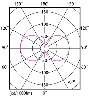
Light Distribution Diagram - 54GC/LED/850 EX39 BB 6/1
