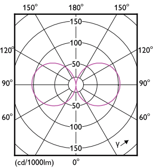
Light Distribution Diagram - 45GC/LED/830 EX39 BB 6/1
