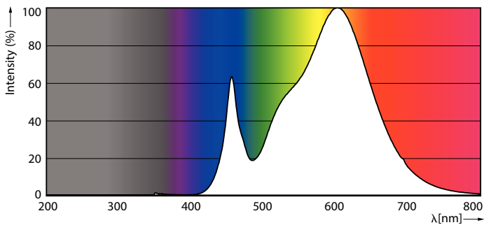
Spectral Power Distribution Colour - 45GC/LED/830 EX39 BB 6/1
