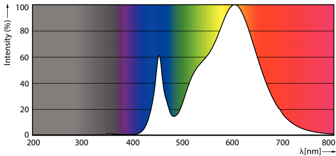
Spectral Power Distribution Colour - 25GC/LED/840/ND E26 BB 6/1
