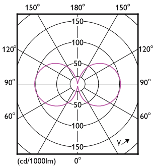
Light Distribution Diagram - 25GC/LED/840/ND E26 BB 6/1
