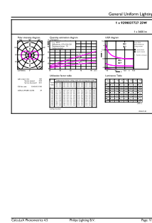
General uniform lighting - 25GC/LED/830/ND E26 BB 6/1
