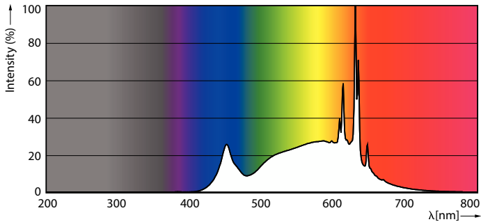
Spectral Power Distribution Colour – 8.5PAR30S/COR/935/F25/D/P/ULW/T20 6/1FB
