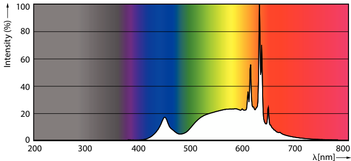
Spectral Power Distribution Colour - 8.5PAR30S/COR/930/F40/D/P/ULW/T20 6/1FB
