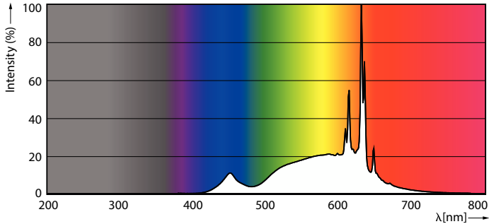
Spectral Power Distribution Colour - 8.5PAR30S/COR/930/F25/D/P/ULW/T20 6/1FB
