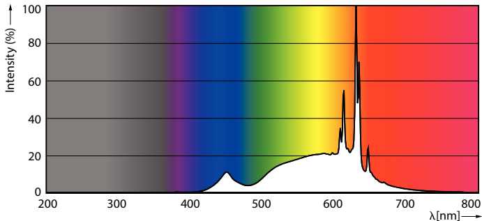
Spectral Power Distribution Colour - 8.5PAR30S/COR/927/F40/D/P/ULW/T20 6/1FB
