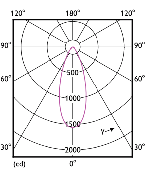
Light Distribution Diagram - 8.5PAR30L/COR/927/F40/D/P/ULW/T20 6/1FB
