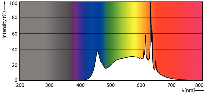
Spectral Power Distribution Colour - 10PAR38/COR/940/F40/DIM/P/ULW/T20 6/1FB
