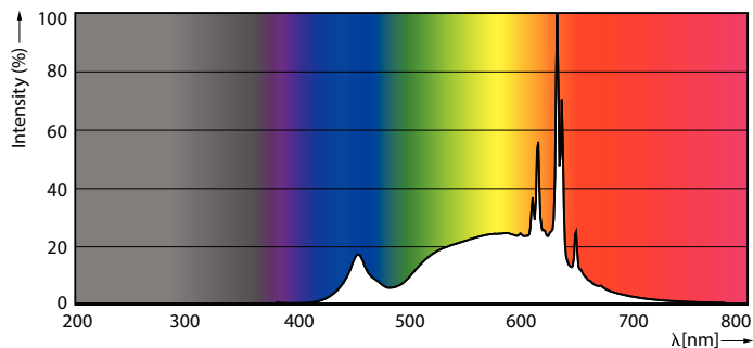
Spectral Power Distribution Colour - 10PAR38/COR/930/F40/DIM/P/ULW/T20 6/1FB
