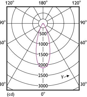
Light Distribution Diagram - 10PAR38/COR/927/F40/DIM/P/ULW/T20 6/1FB
