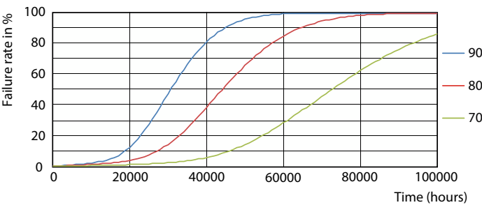
Life Expectancy Diagram - 16.5T8/MAS/48-840/MF25/P/DIM 25/1
