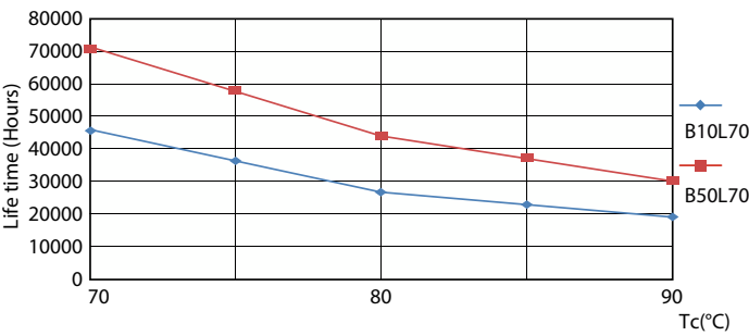
Life Expectancy Diagram - 16.5T8/MAS/48-840/MF25/P/DIM 25/1
