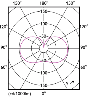
Light Distribution Diagram - 19GC/LED/840/ND E26 BB 6/1
