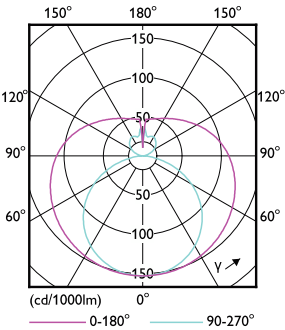
Light Distribution Diagram - 14.5T8/CNG/48-840/MF18/G 25/1
