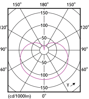
Light Distribution Diagram - 16A21/PER/930/P/GU24/DIM 4/1FB T20
