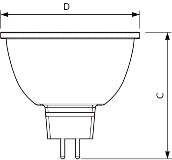
6.3MR16/LED/F25/930/D/EC/12V T20 10/1FB
