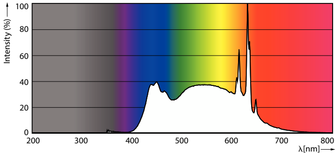
Spectral Power Distribution Colour - 3.5G25/PER/UD50/CL/G/E26/D 4/2PFT20
