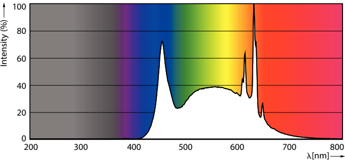
LEDbulb T20 16,6W A19 E26 950 FR-POC
