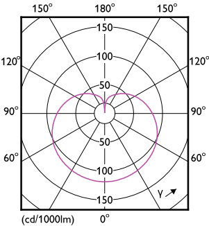
Light Distribution Diagram - 18.5A21/PER/927/FR/P/E26/3WAY/T20 4/1PF
