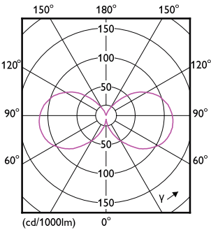
Light Distribution Diagram - 4A19/PER/GREEN/G/E26/ND 4/1PF
