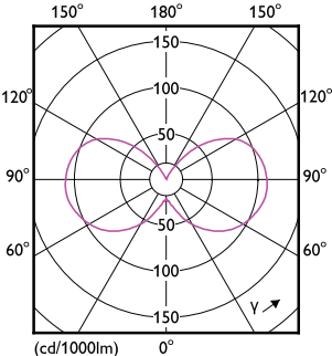
Light Distribution Diagram - 3.5BA11/PER/UD/CL/G/E26/WGD 6/3PF T20
