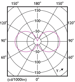
Light Distribution Diagram - 2.3BA11/PER/UD/CL/G/E12/WGD 6/3PFT20
