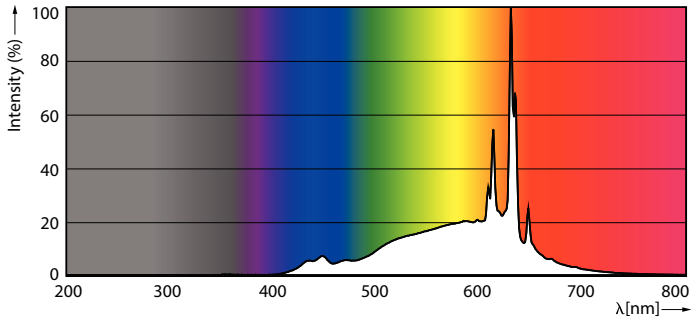
Spectral Power Distribution Colour - 2.3BA11/PER/UD/CL/G/E12/WGD 6/3PFT20
