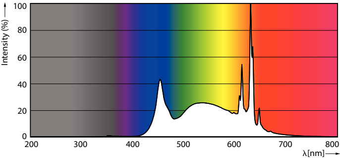
Spectral Power Distribution Colour - 5.5ST19/VIN/950/E26/CL/G/SP D 4/1PF T20
