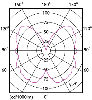
General uniform lighting - 5.5A19/VIN/927/E26/CL/G/SP DIM 1PF T20
