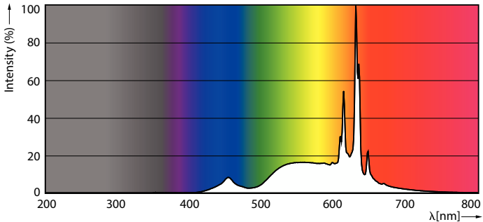
Spectral Power Distribution Colour - 5.5A19/VIN/927/E26/CL/G/SP DIM 1PF T20
