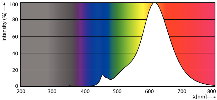
Spectral Power Distribution Colour - 3.5T10/VIN/820/E26/Amber/G/SP D 4/1PFT20
