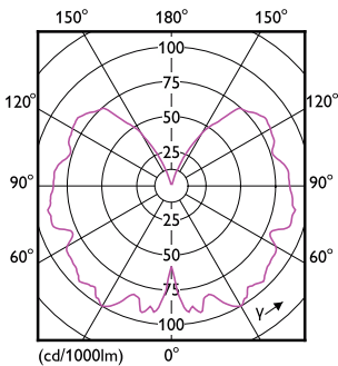
Light Distribution Diagram - 3.5T10/VIN/820/E26/Amber/G/SP D 4/1PFT20
