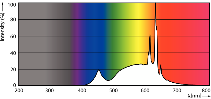
LEDbulb G6 13,5W A19 E26 930 FR-POC
