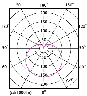
LEDbulb G6 A19 5W E26 950 FR-LDD
