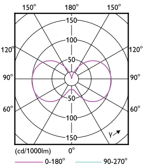
LEDTForce LS 450W Corncob EX39-LDD
