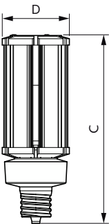
54CC/LED/850/LS EX39 G3 BB 3/1
