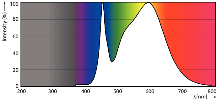
Spectral Power Distribution Colour - 165HB/LED/840/D WB UDL BB G2 4/1
