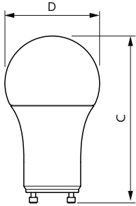
8.8A19/PER/930/P/E26/DIM
