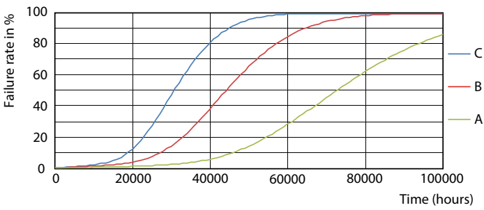
LEDtube_70K_FailureRate-LED
