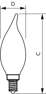
Candle BA11 4.5-40W 300lm 2000K D Amber
