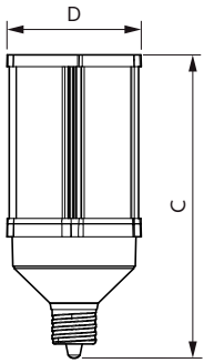
Corn lamp LED 100W EX39 830 CL
