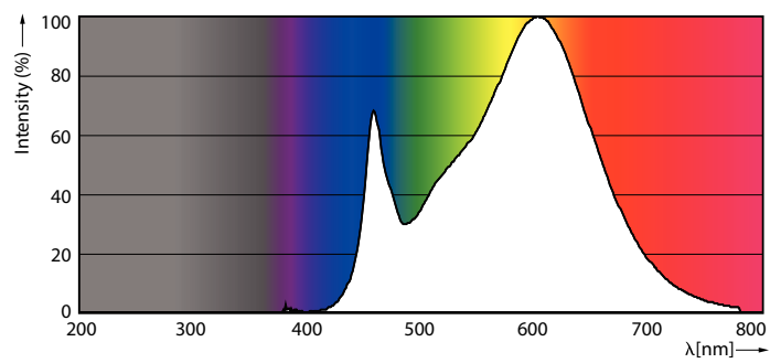
Corn lamp LED 100W EX39 830 CL
