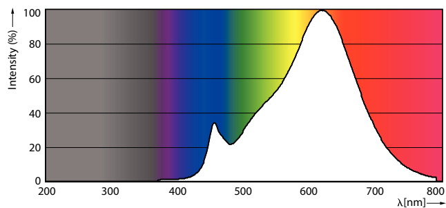
LEDbulb 927 CL-POC
