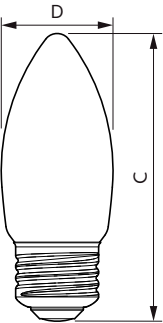
Candle B11 120V5.5-60W500lm5000KE26DCL
