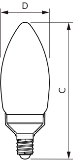
Candle B11120V 5.5-60W500lm5000KE12DCL
