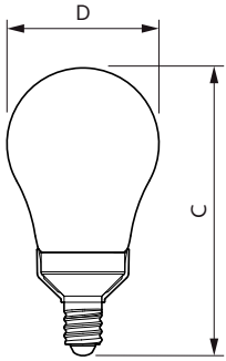
BulbA15120V3.8-40W350lm2700-2200KE12DCL
