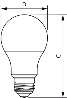
Bulb A60 120V 10-60W 800lm 5000K E26 ND
