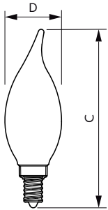
Candle BA11 4.5-40W 300lm 2000K D Amber
