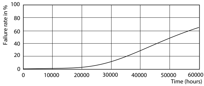
LEDtube 1200mm 14W G13 2000lm
