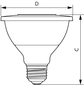
PAR30S 120V 12-90W 950lm 40D 3000K E26
