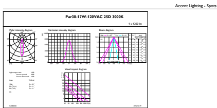
LEDspot PAR38 E26 25°
