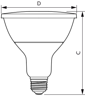
PAR38 120V 17-120W 1250lm 25D 3000K E26
