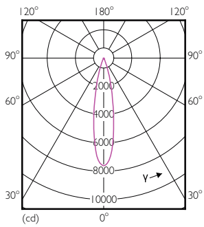
LEDspot PAR38 E26 25°
