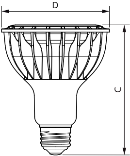
PAR30L 27.5-W 2000lm 25D 3000K E26 ND
