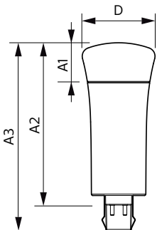
PLED PLC-V 5-13W 550lm 3000K G24q
