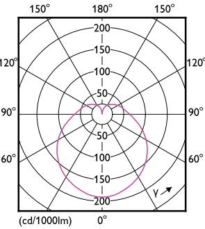
LEDtube PLC 13V 5W GX23-2 827 15D ND
