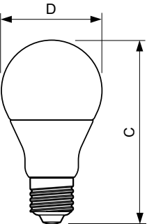
Bulb A21 120V 18-100W 1600lm 5000K E26ND
